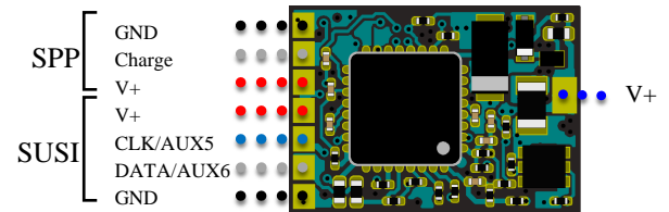
Top view – solder pads description
