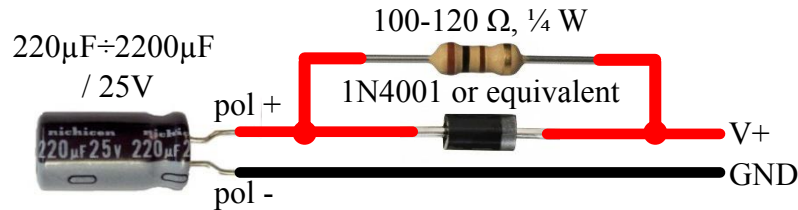
Figure 144: Buffer capacitor connection
