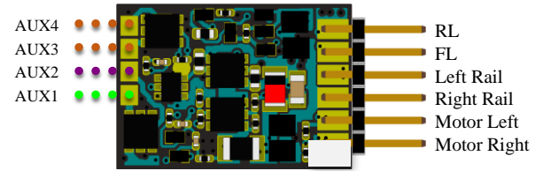
Micro 6P, 6P90 and 6P90R – Bottom view
