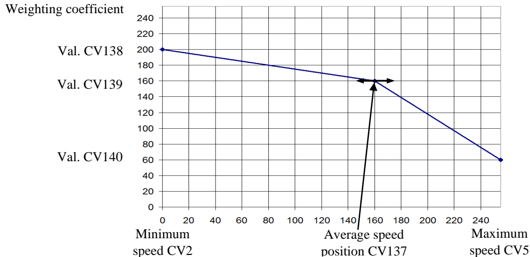
Figure 12: Load compensation
