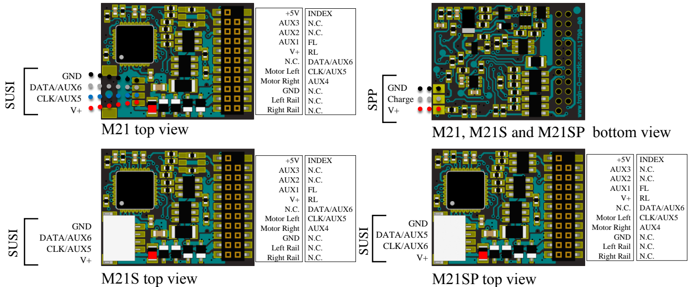
Figure 4: Lokommander II Mini M21, M21S and M21SP
