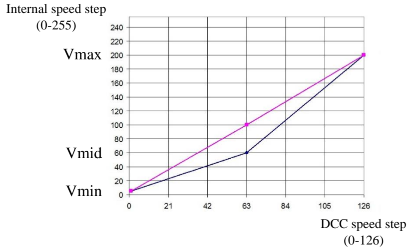
Figure 7: 3 points speed adjustment
